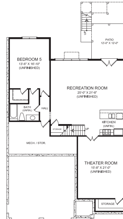
BASEMENT
